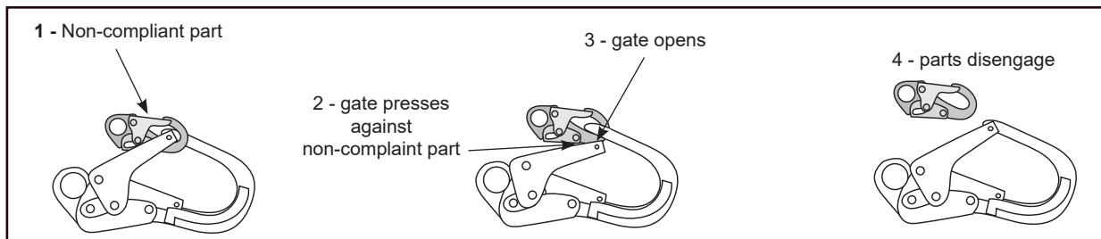
FIGURE 4 - UNINTENTIONAL DISENGAGEMENT
