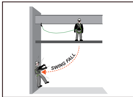
FIGURE 3 - SWING FALLS
